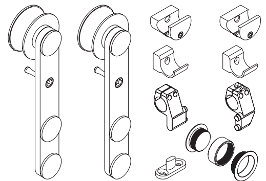
No. ORF100 HANGER SET
